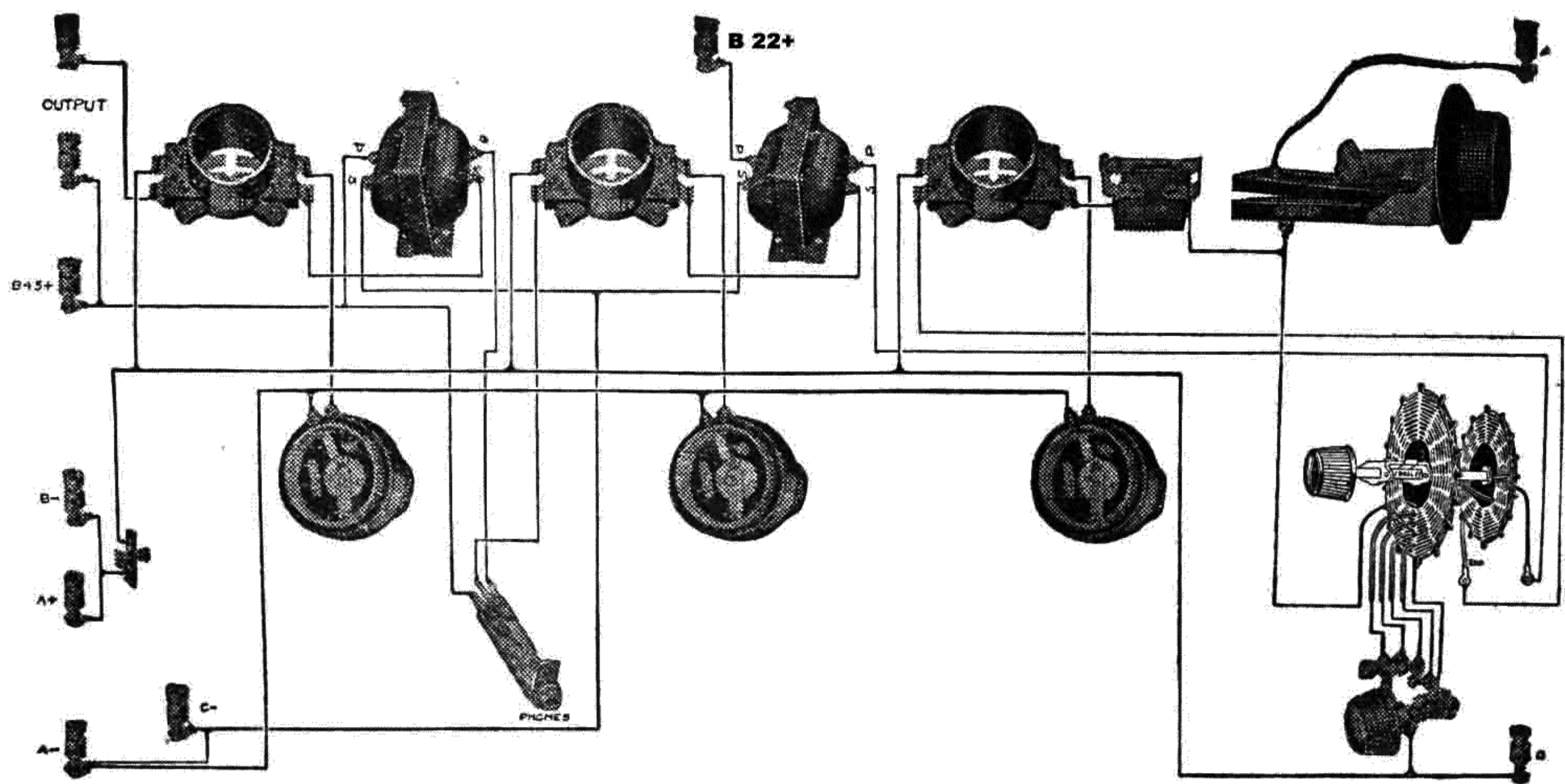
Crosley 3B or 3C Regenerative Detector and Two-step Amplifier Receiver
