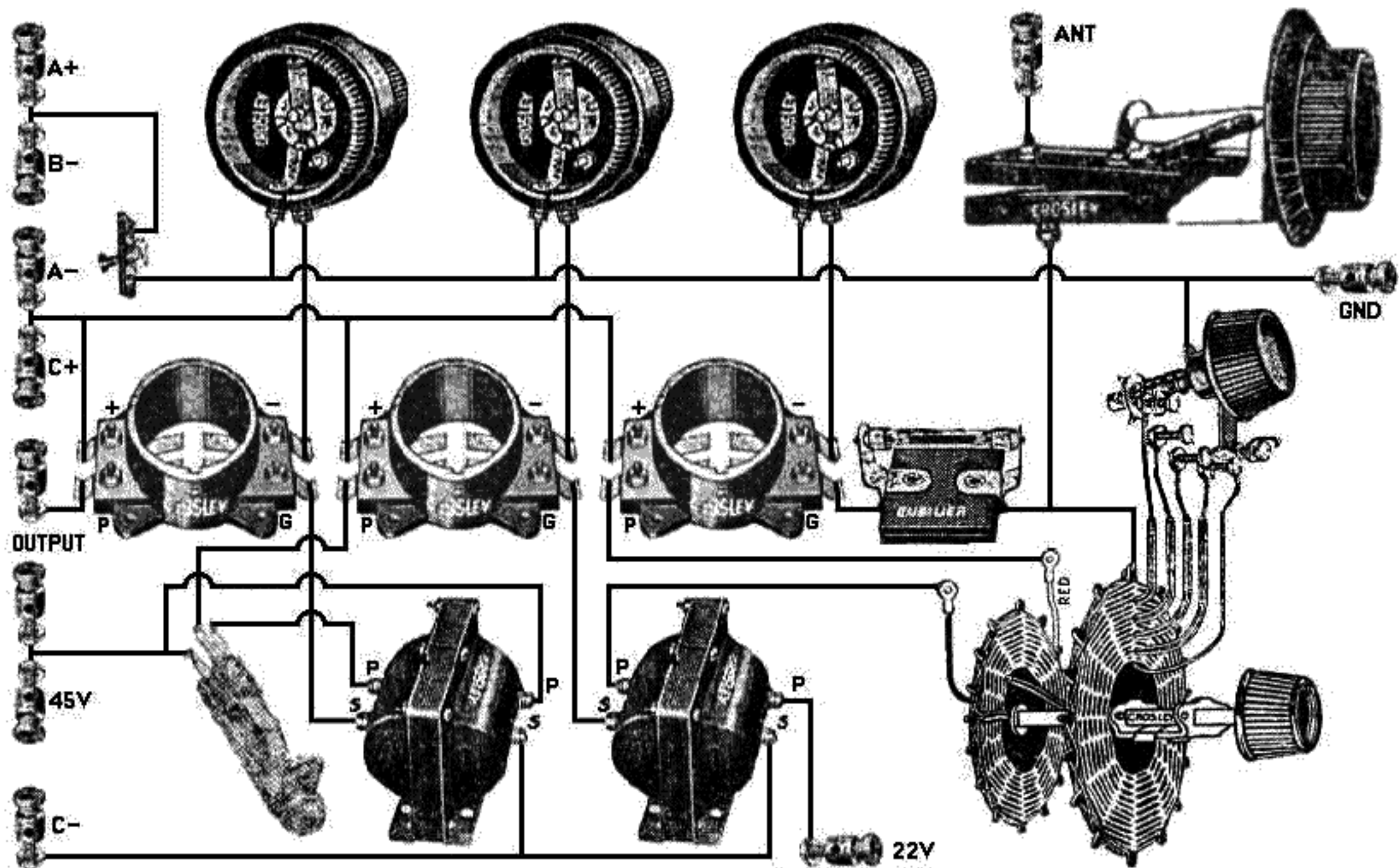
Crosley 3B or 3C Detector & Two-step Amplifier Receiver
