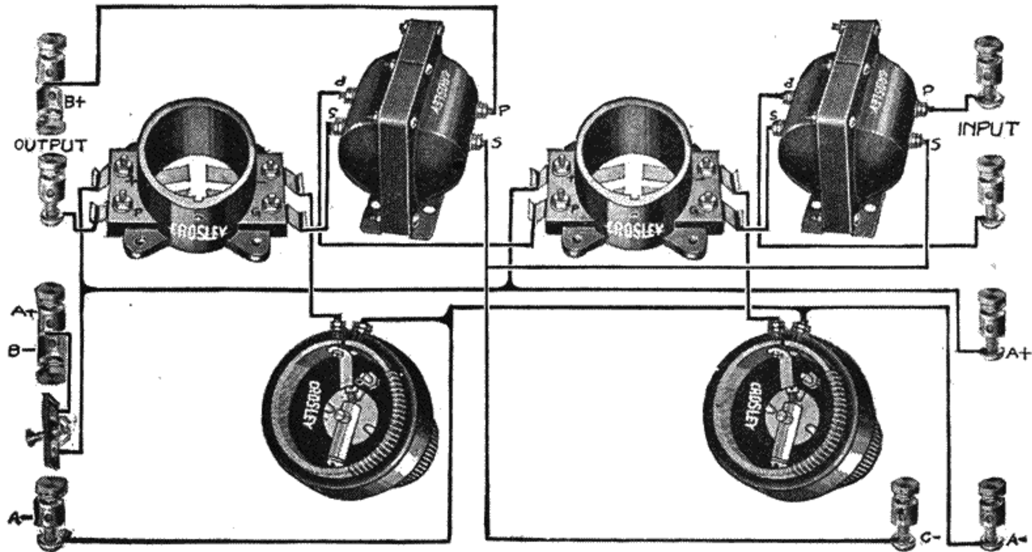
Two-Step Audio Frequency Amplifier Circuit
